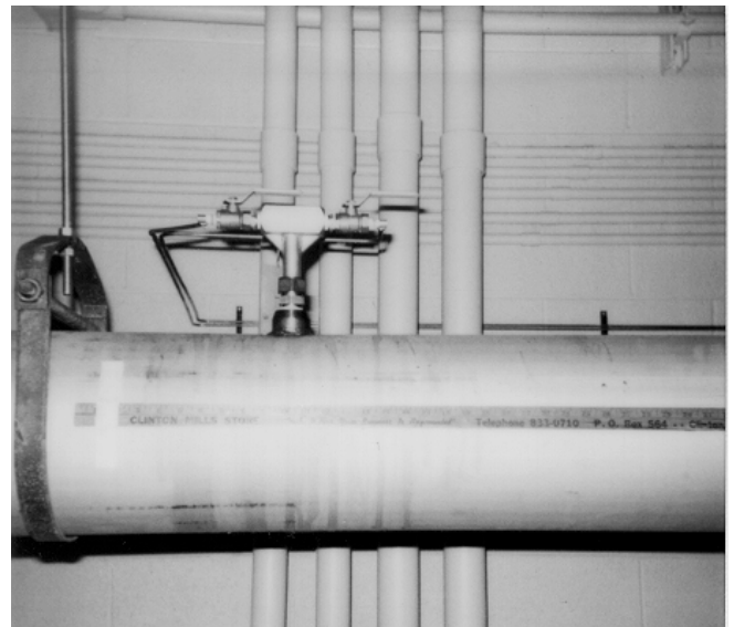
Verabar® installed on 10" compressed air main header (27,500 SCFM, 95 PSI, 85°F). This is one of 18 sensors in service at Clinton Mills, a large textile plant in Clinton, South Carolina.
